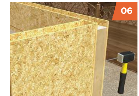
06 Corner joints are nailed together to ensure structural strength.
