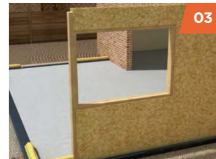
03 Subsequent panels are installed with specified window and door openings.
